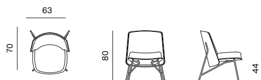
EASY CHAIR dimensions 63 x 70 x 80 cm
