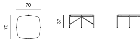
LOW TABLE dimensions 70 x 70 x 37 cm
