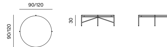
LOW TABLE dimensions \varnothing 90 , \varnothing 120 x 30 cm
